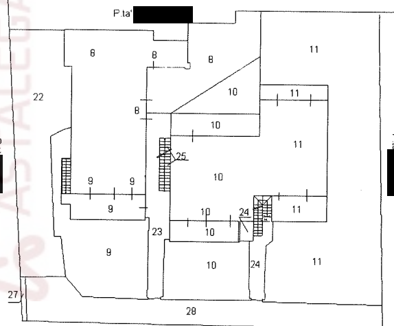
PIANO TERRA
