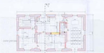
PIANO TERRA IN VARIANTE
